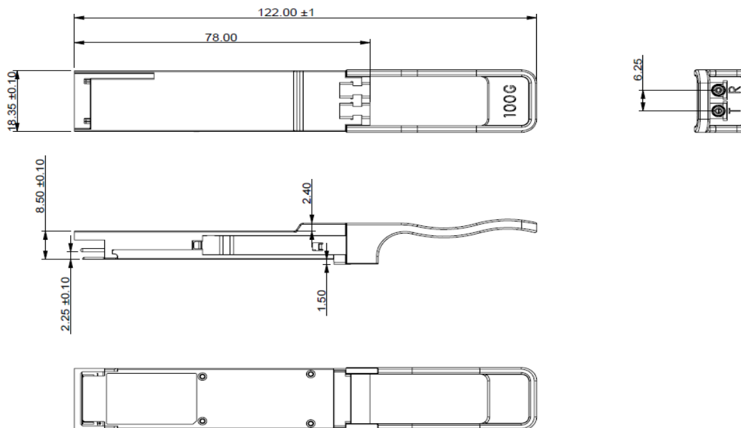
Figure 4. Mechanical Outline
